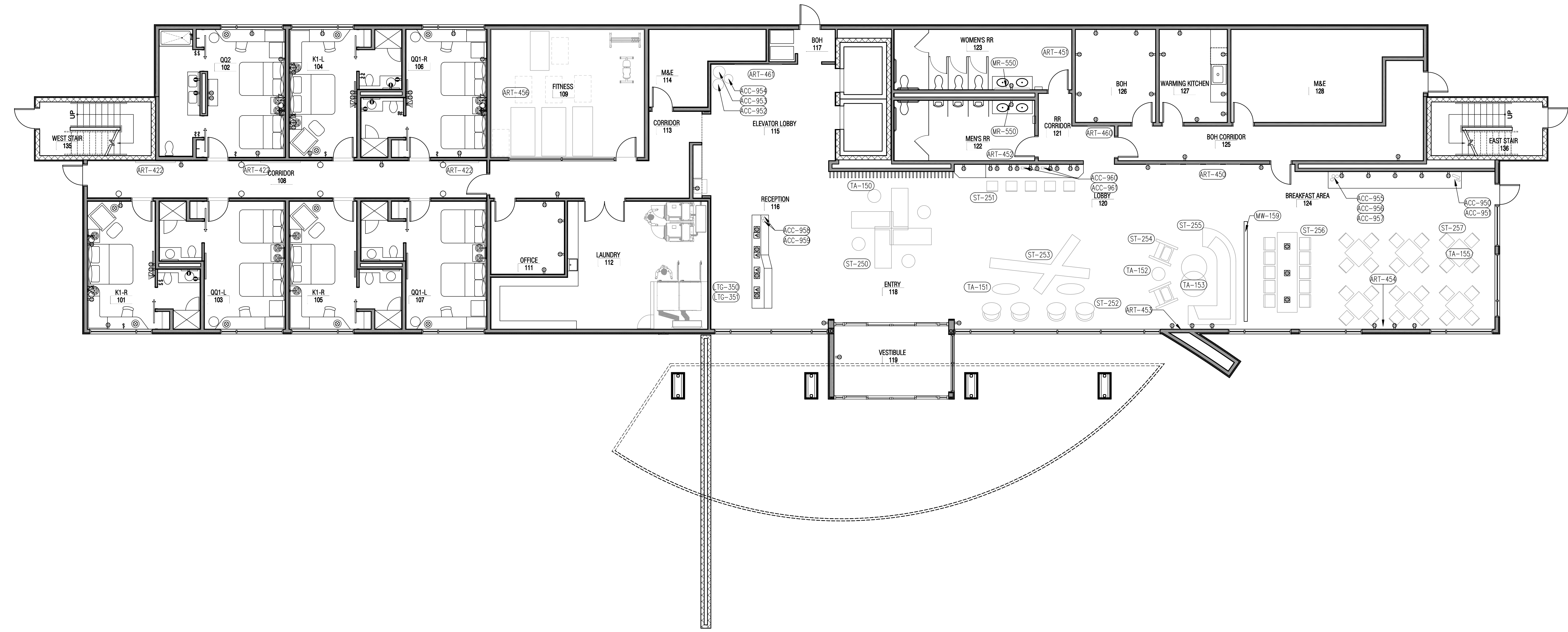
FURNITURE PLAN LEVEL 1 1/8" = 1'-0" 1
